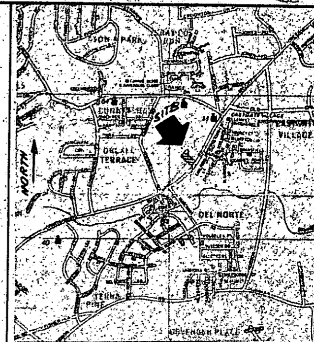
LOCATION MAP
