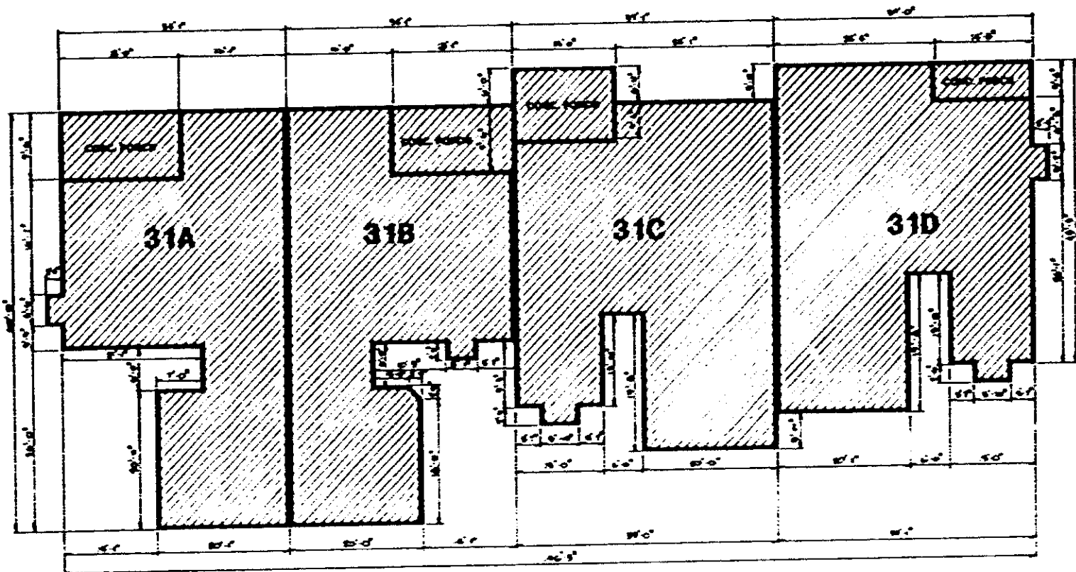
FOUNDATION PLAN
