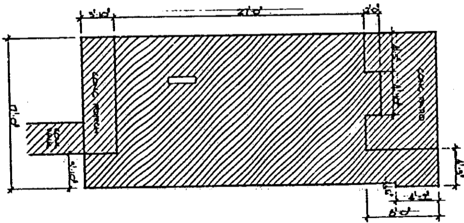
FOUNDATION PLAN
