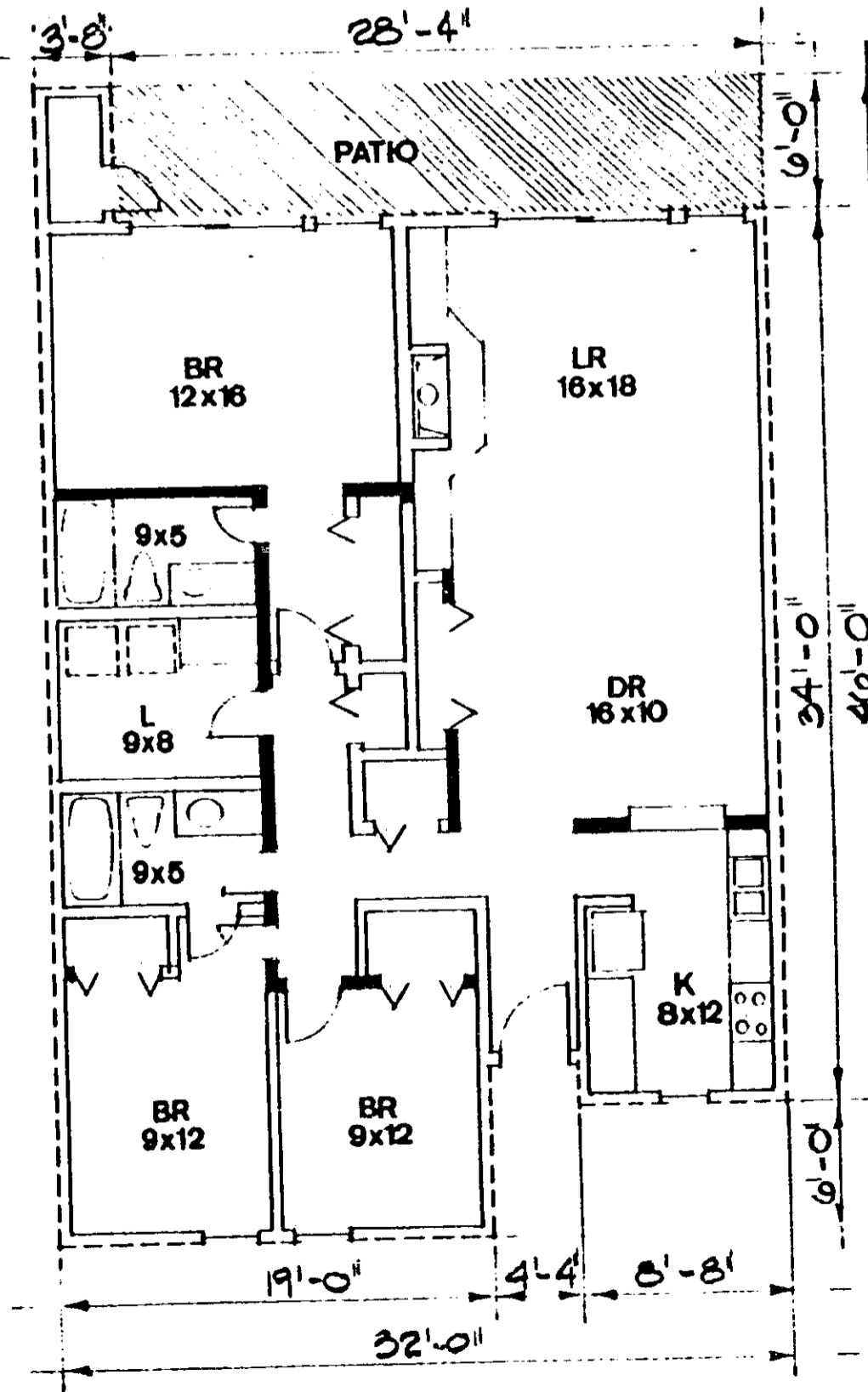
FLOOR PLAN
