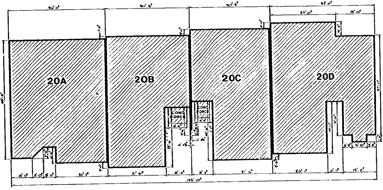
FOUNDATION PLAN
