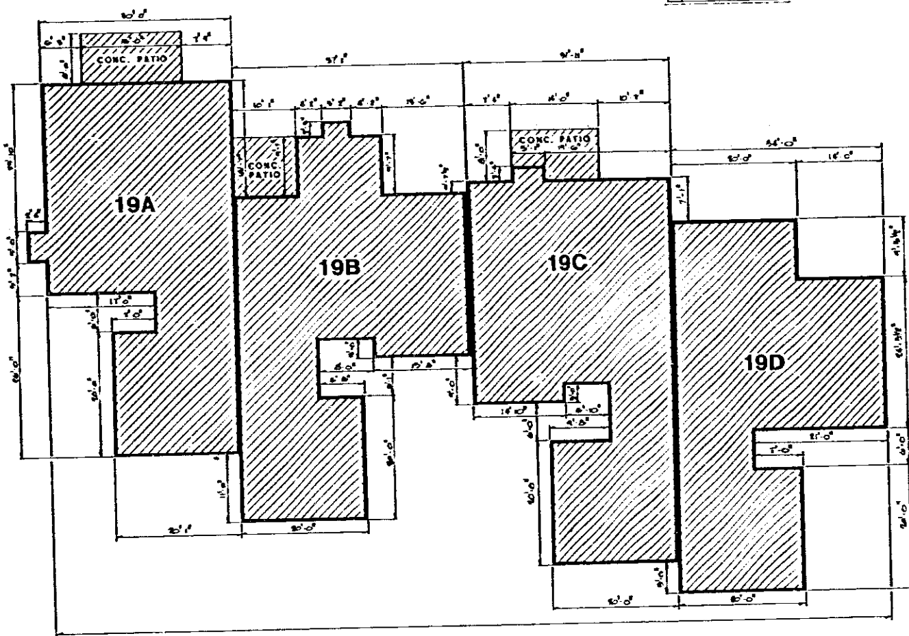
FOUNDATION PLAN
