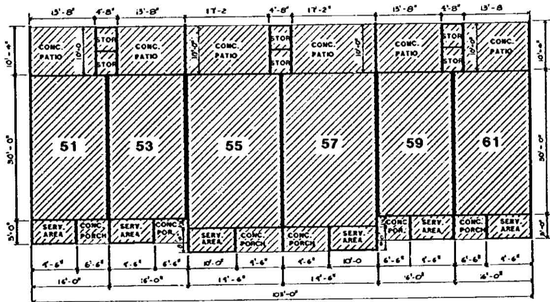
FOUNDATION PLAN
