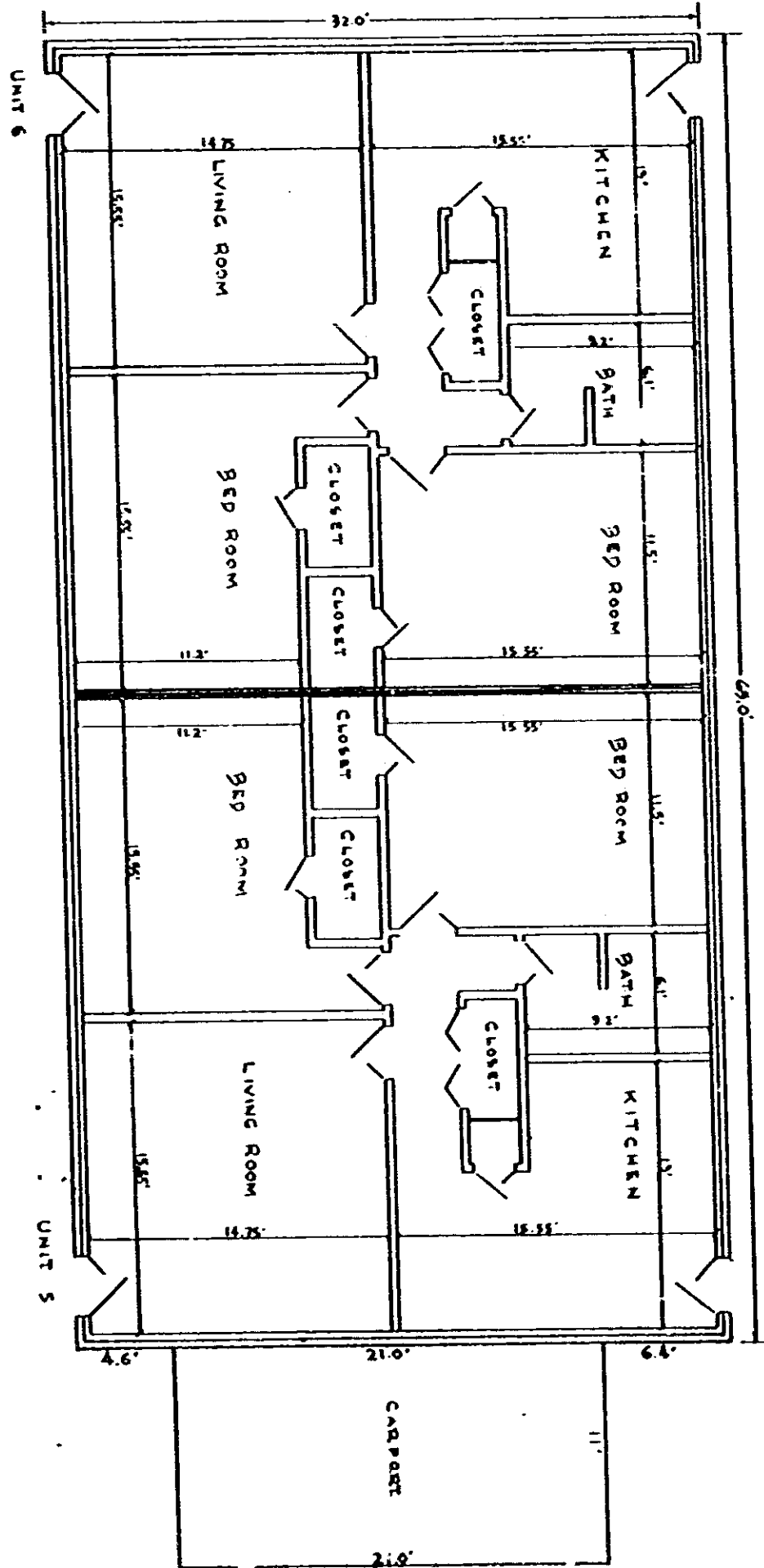
FLOOR PLAN
