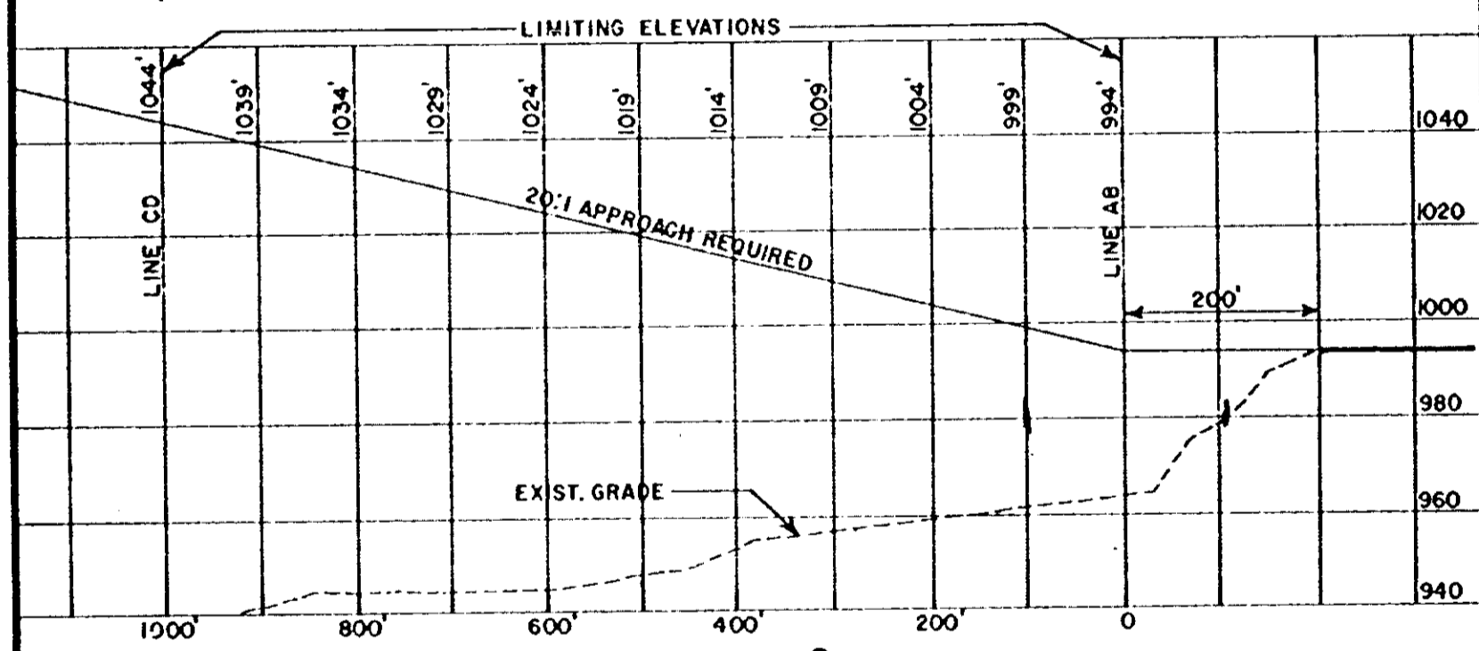
PROFILE ALONG R/W \text{\textcircled{C}} SCALE: VERT. 1" = 40' HORZ. 1" = 200'
