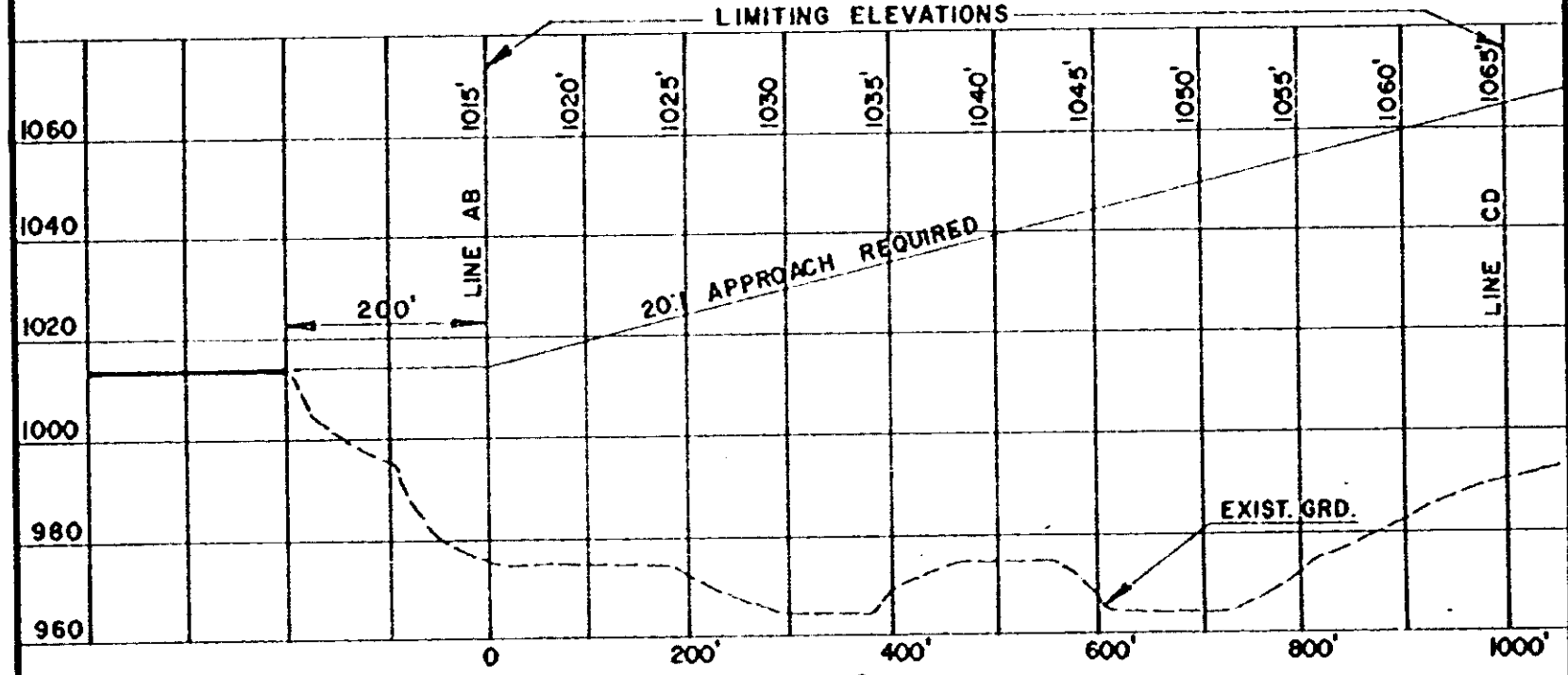
PROFILE ALONG R/W
