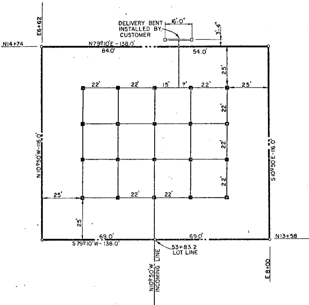
DETAILS OF SUBSTATION LOT SCALE: 1" = 30'
