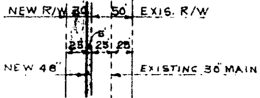
PLAN SECTION SCALE 1"=100'
