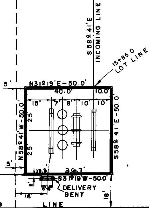
DETAILS OF SUBSTATION LOT SCALE 1" = 30'
